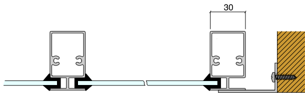
Toppvy fast B-parti
