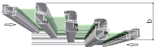
4-delat parti, b=119.5 mm. Stolpbredd=106.5 mm.
