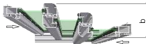
3-delat parti, b=94mm. Stolpbredd= 81mm.
